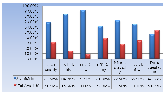
Fig. 1: The adherence to the seven main software quality criteria
